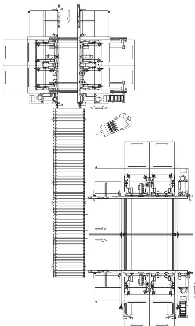
Sample layout: Angular system ProfiShape
