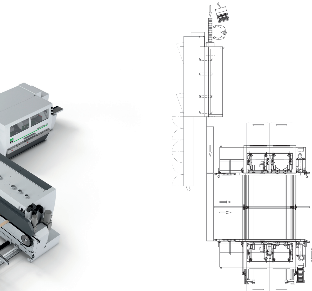
Sample layout: Combination of double-end tenoner ProfiShape T4W and Powermat P 1500
