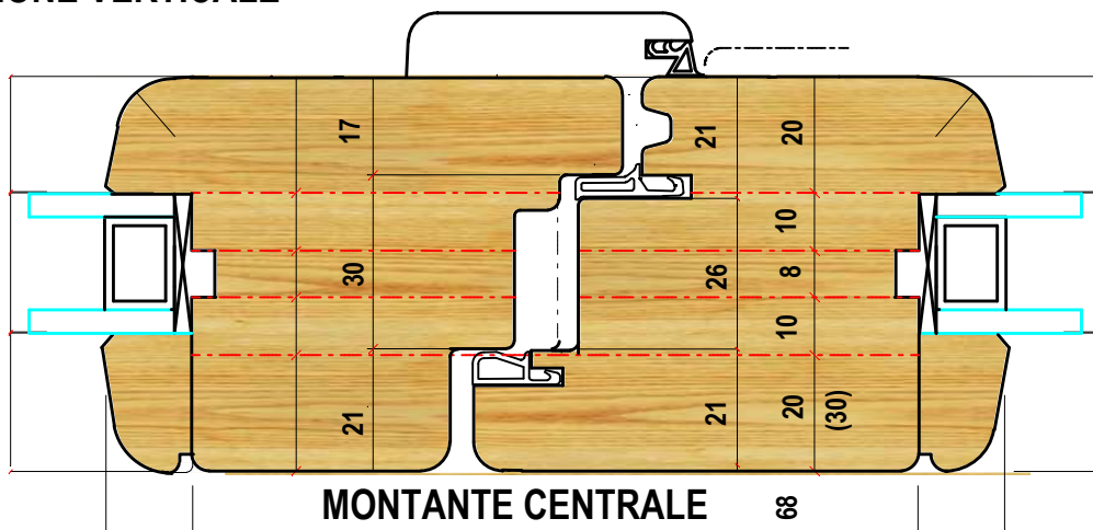
PORTA BALCONE
