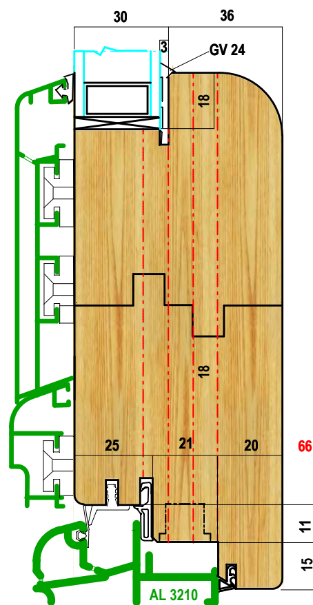
PORTA BALCONE
